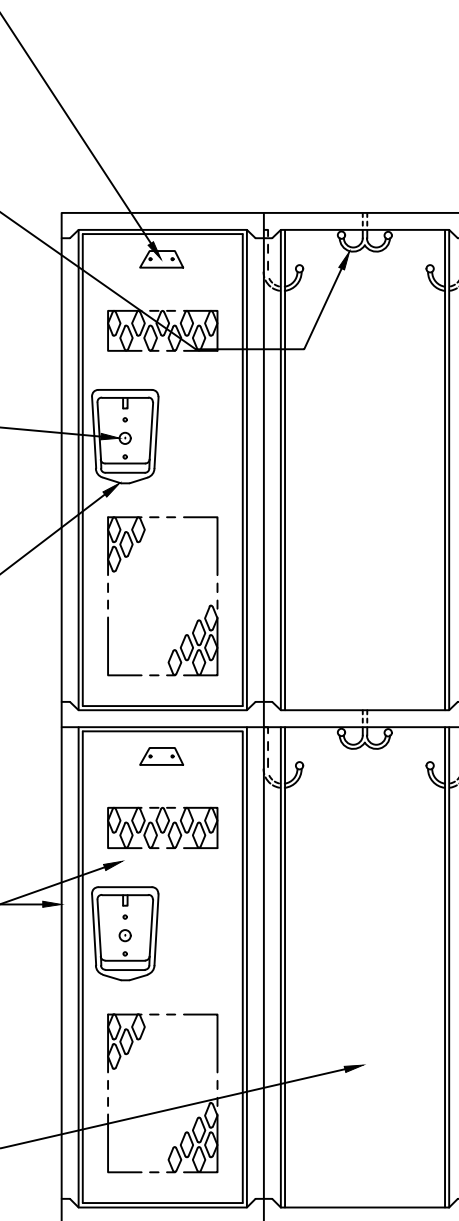
12 1/16" LOCKER ELEVATION
