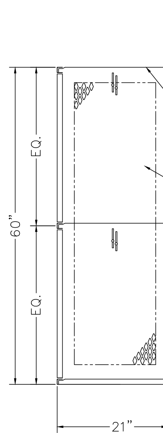
LOCKER SECTION
