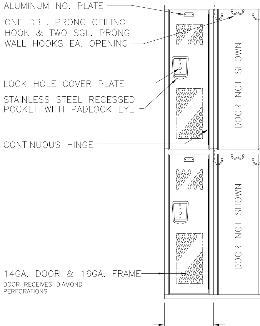
ELEVATION SECTION @ WALL 72" HIGH DOUBLE TIER ALL-WELDED LOCKER 12" & 15" WIDE, ALLOW 1/16" CREEPAGE PER FRAME TYPICAL FOR 12", 15", 18", 21" & 24" DEEP
