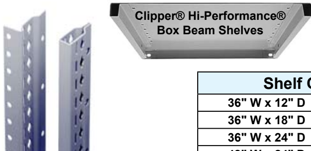
Angle posts (left) at rear of units. Box Posts (right) at front of units.
