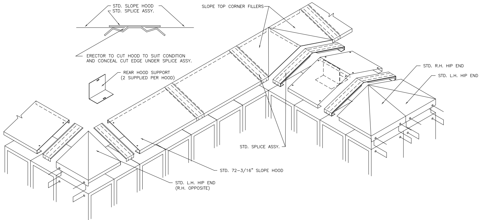
SLOPE HOOD DETAIL W/ HIP ENDS
