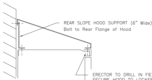
DETAIL OF SINGLE ROW SLOPE HOOD AT WALL
