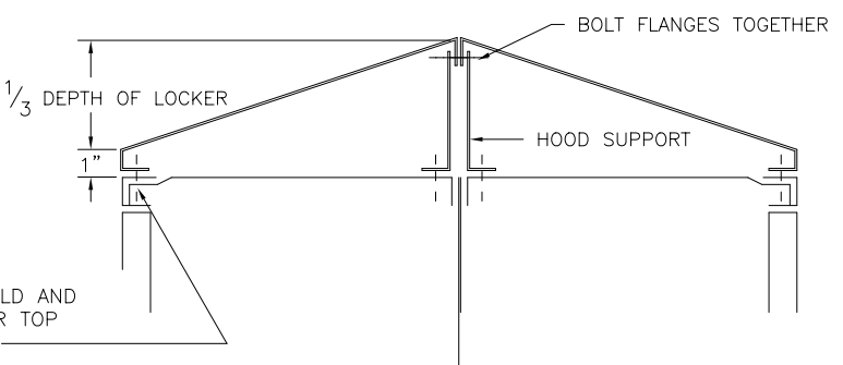
DETAIL OF DOUBLE ROW SLOPE HOOD
