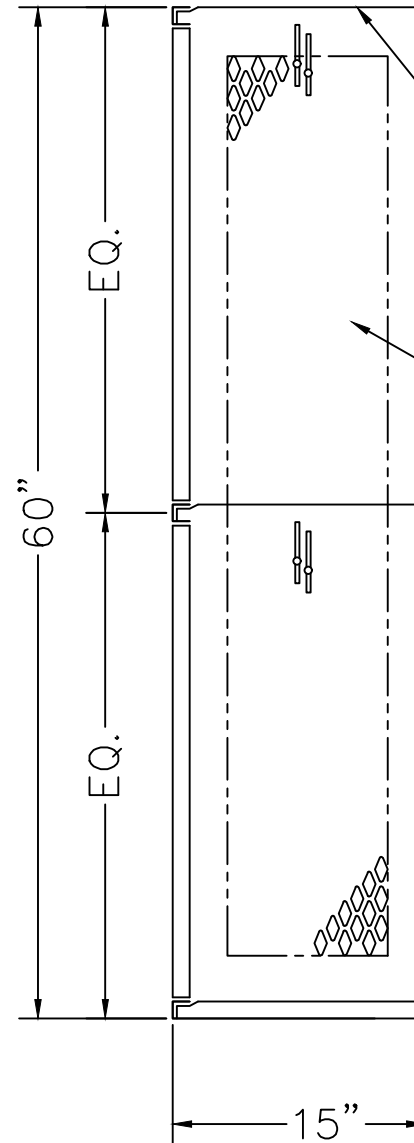
LOCKER SECTION
