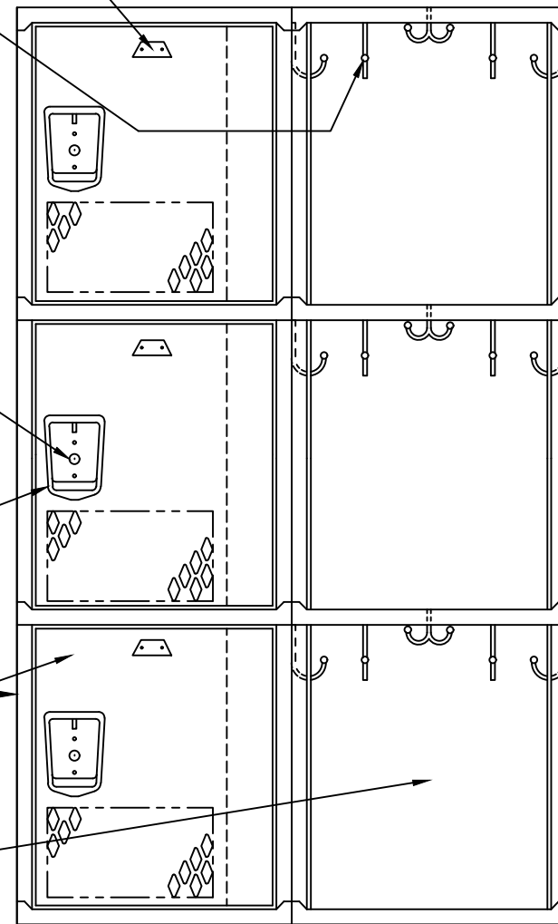
18 1/16" LOCKER ELEVATION
