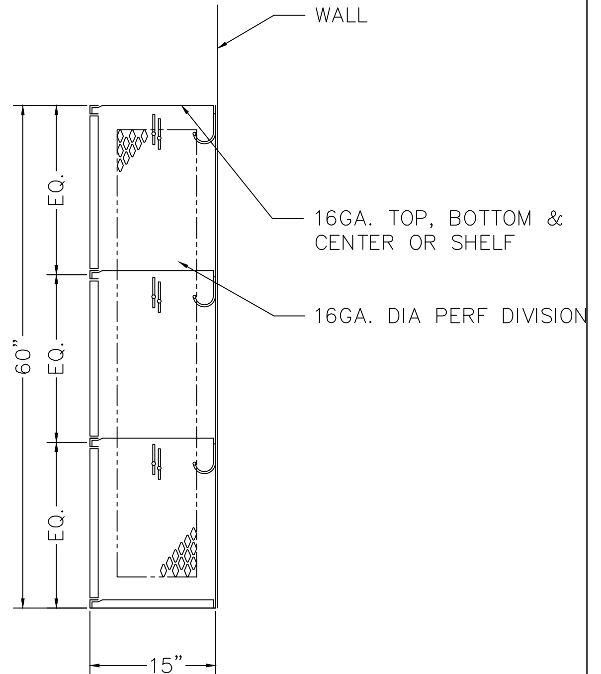
60" 15" LOCKER SECTION
