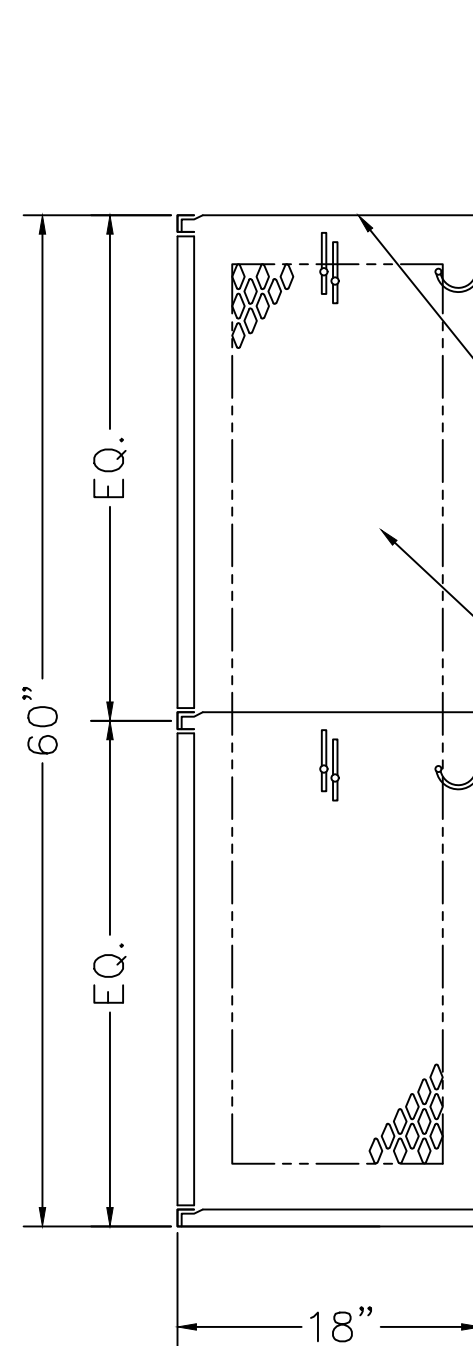
LOCKER SECTION
