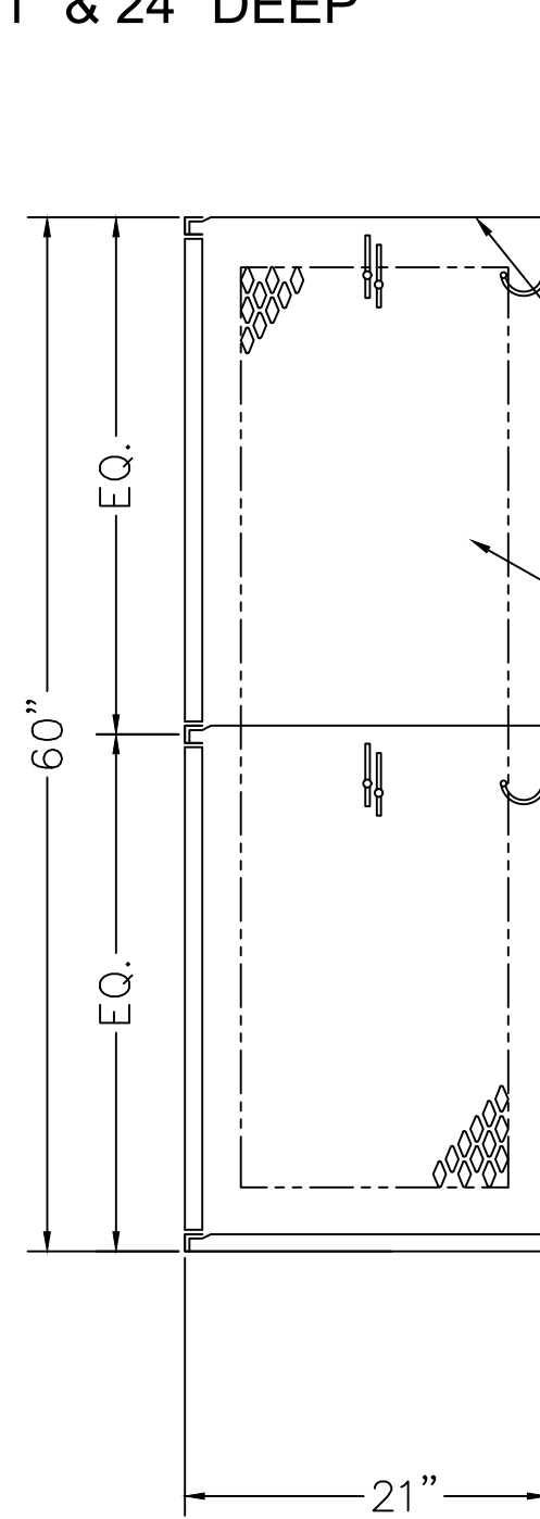
LOCKER SECTION
