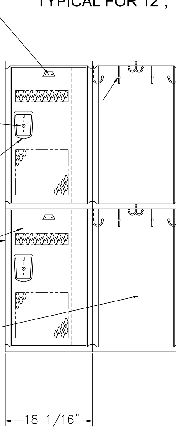
LOCKER ELEVATION
