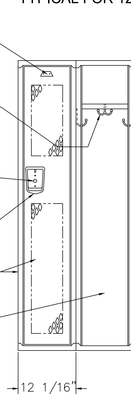
LOCKER ELEVATION
