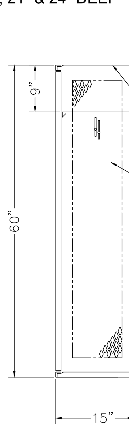
LOCKER SECTION
