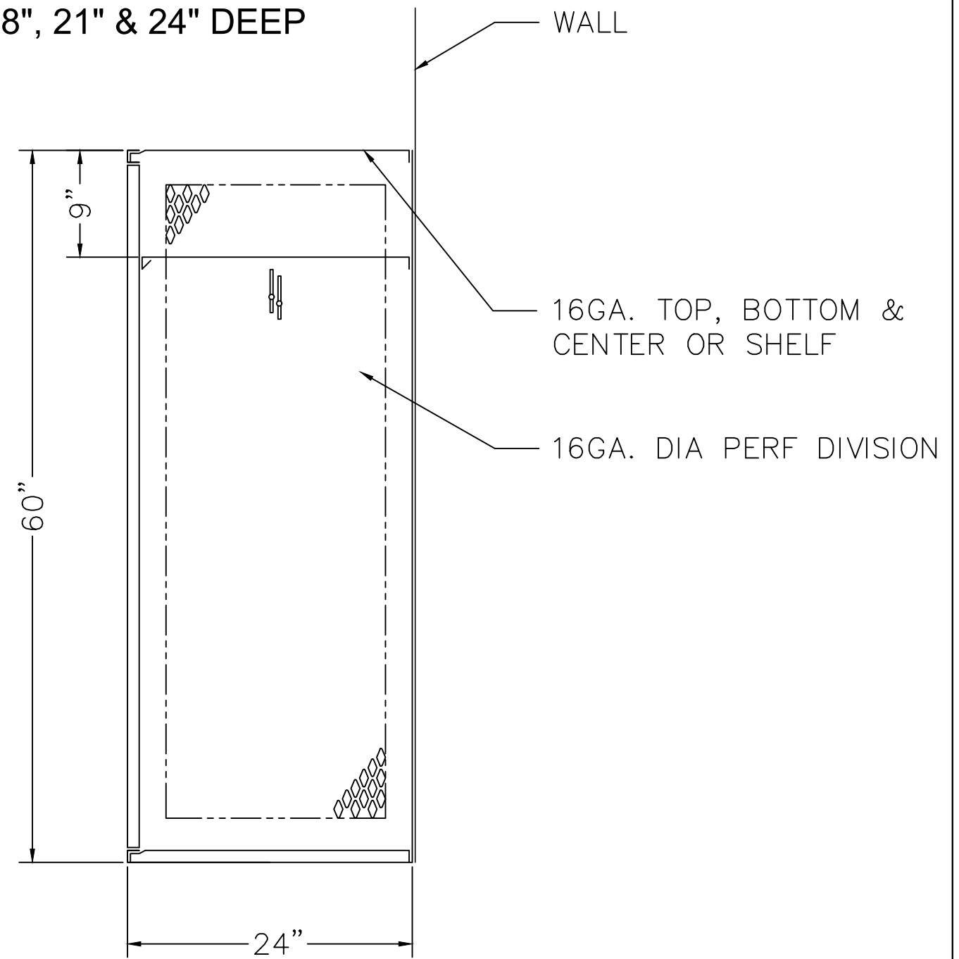
LOCKER SECTION
