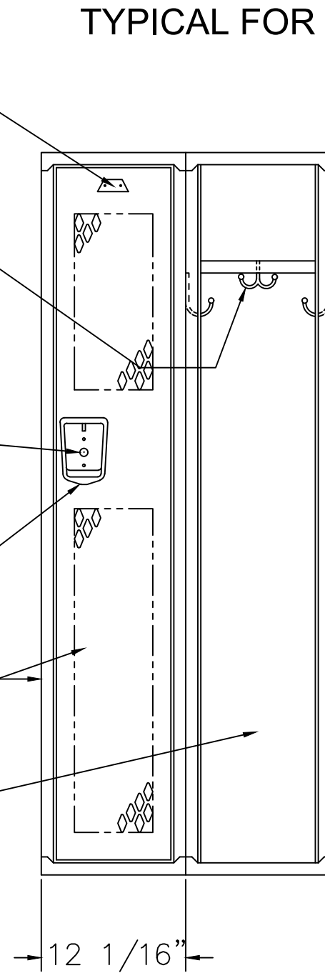
LOCKER ELEVATION
