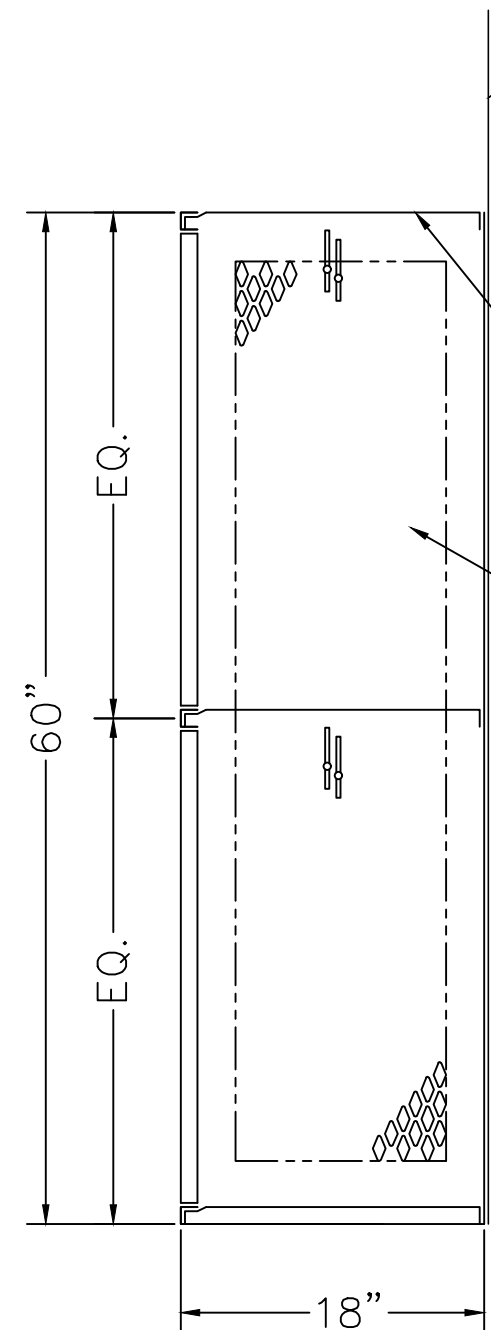
LOCKER SECTION
