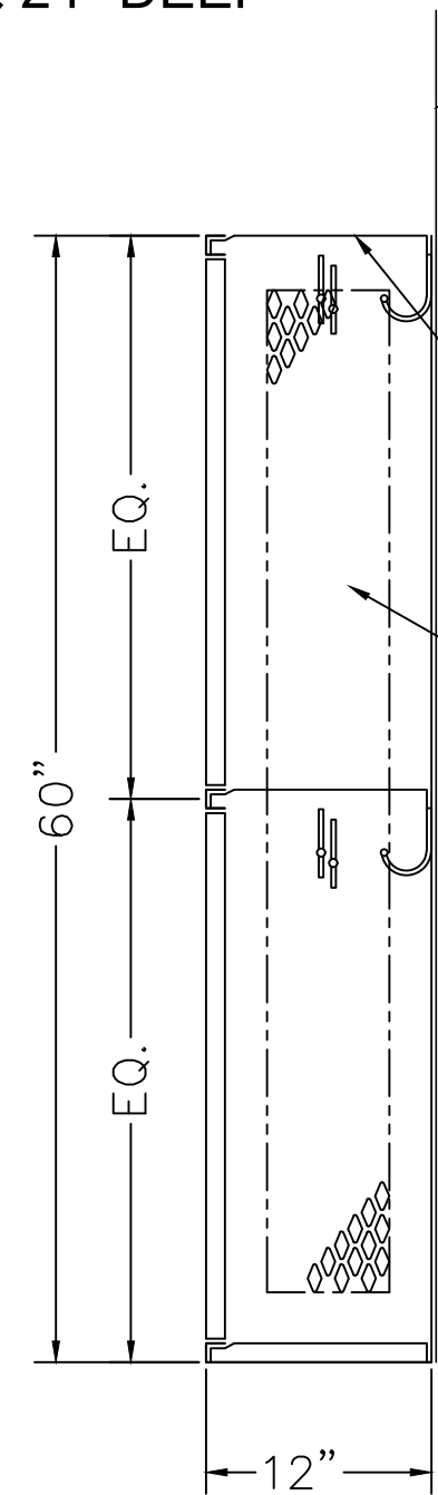
LOCKER SECTION
