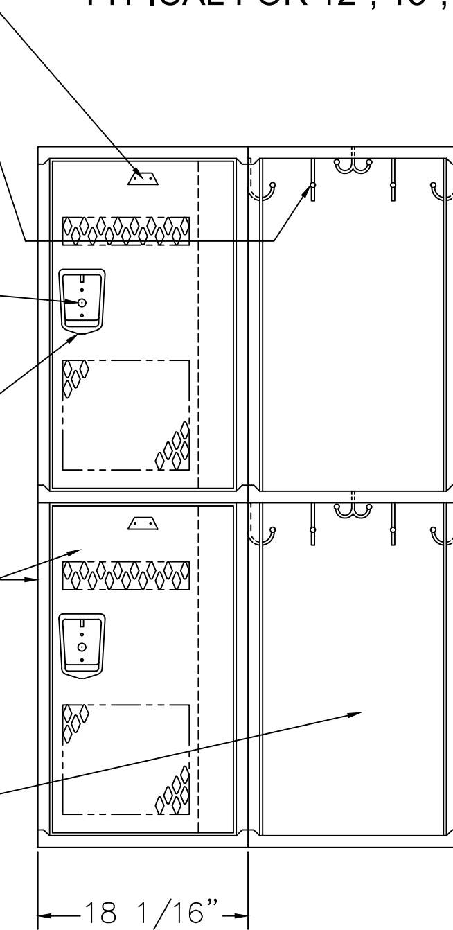
LOCKER ELEVATION
