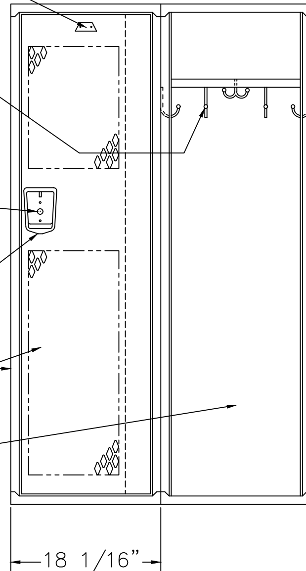
LOCKER ELEVATION
