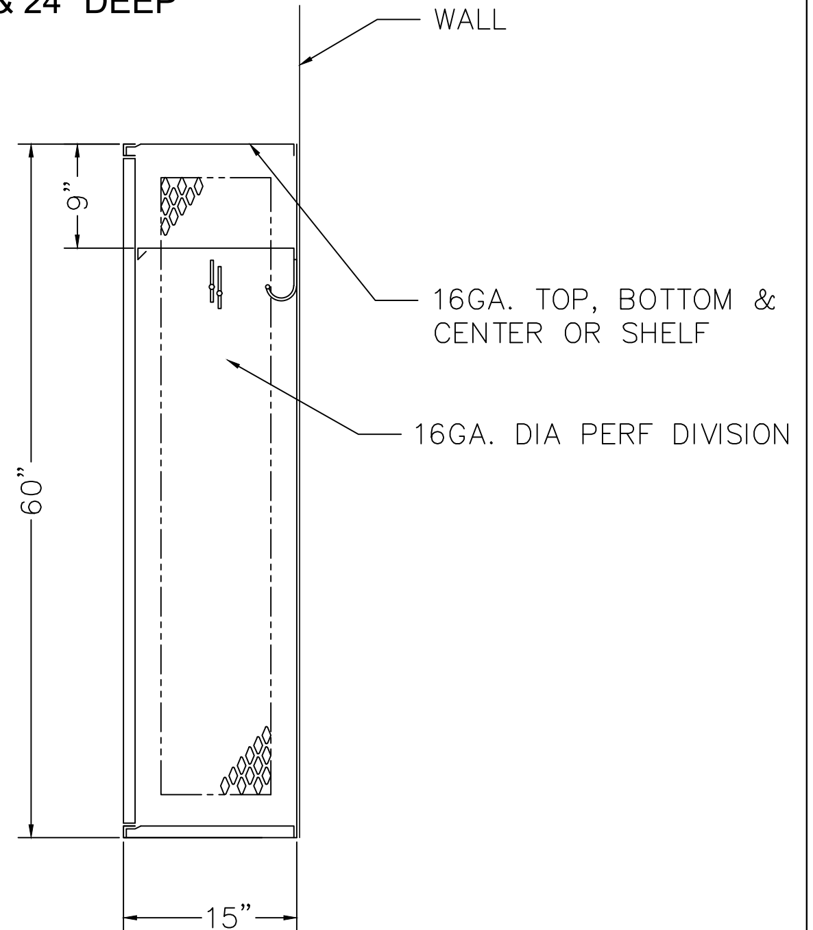
LOCKER SECTION
