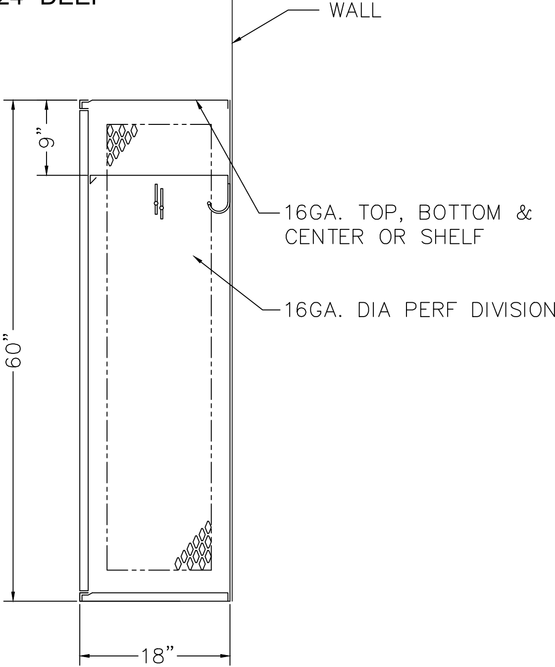
LOCKER SECTION
