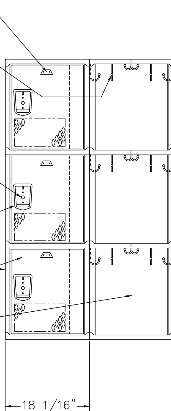
LOCKER ELEVATION
