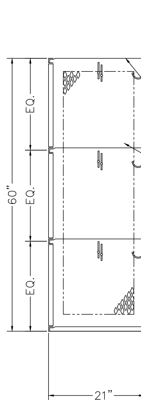
LOCKER SECTION
