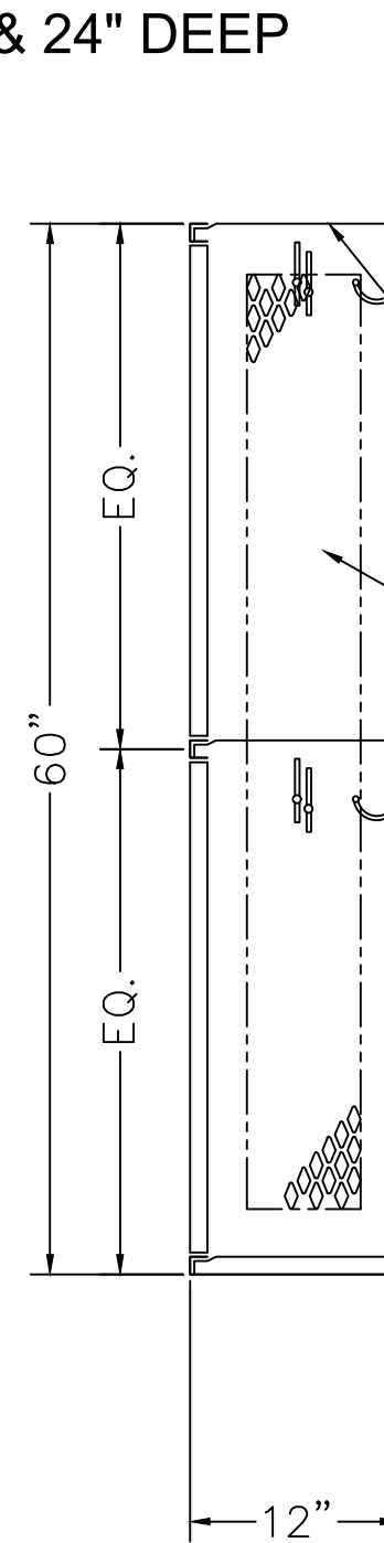
LOCKER SECTION
