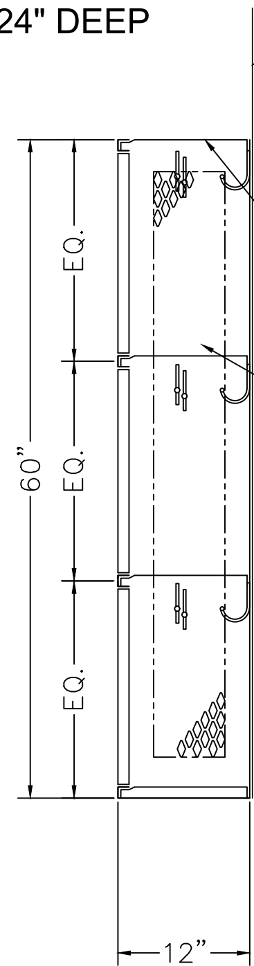
LOCKER SECTION
