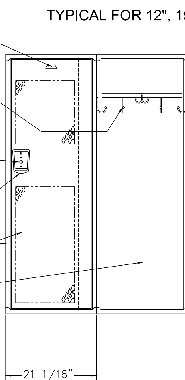
LOCKER ELEVATION
