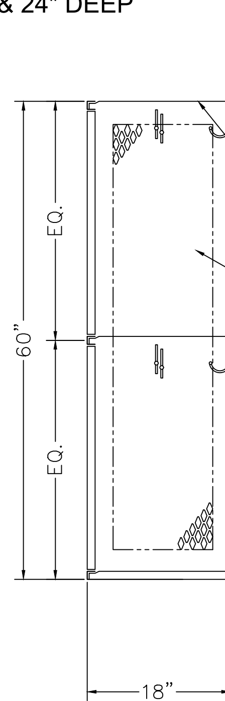
LOCKER SECTION
