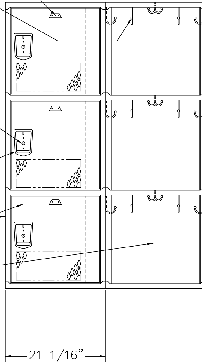
LOCKER ELEVATION
