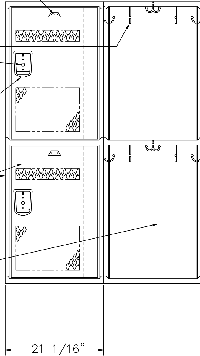
LOCKER ELEVATION
