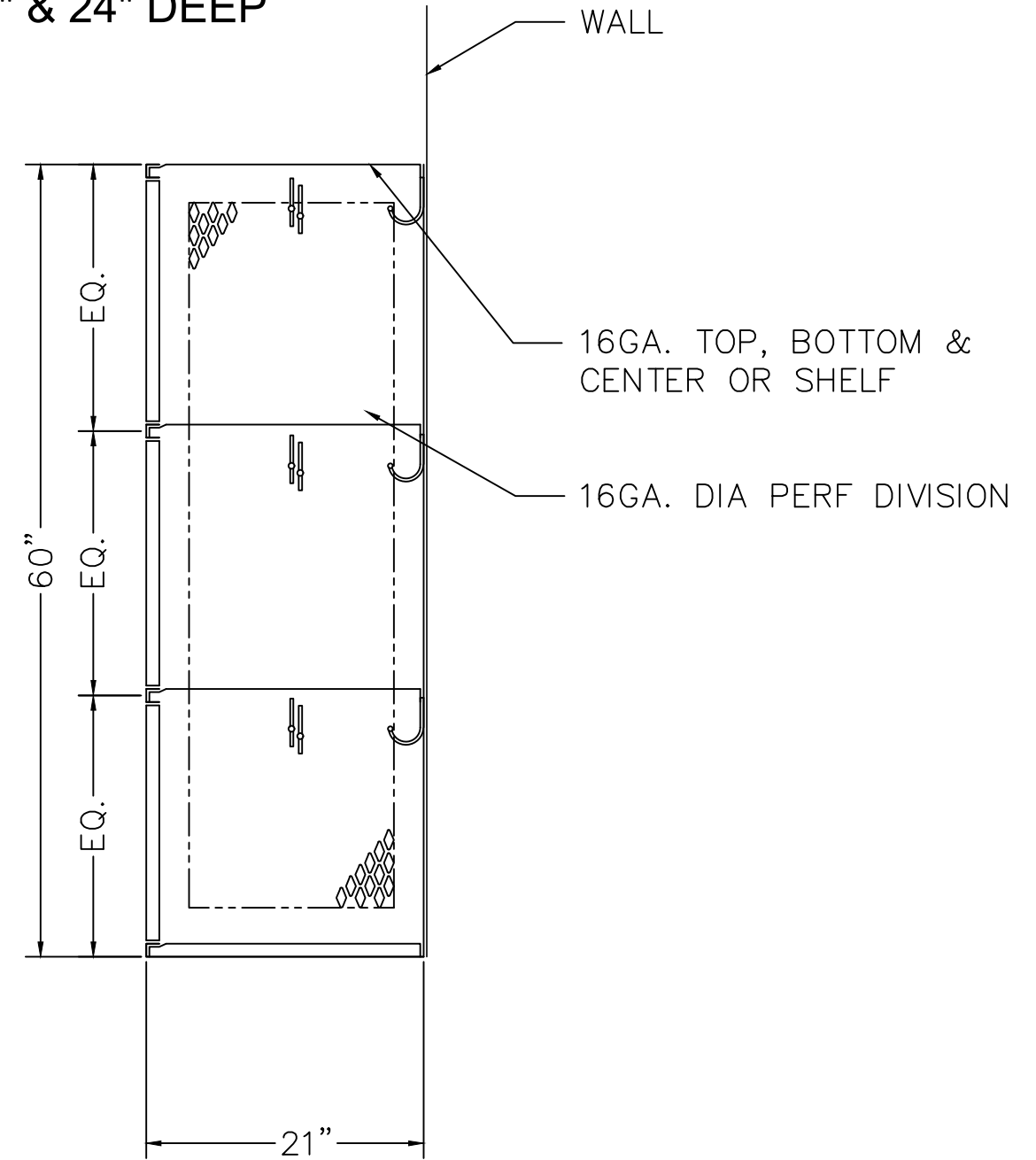
LOCKER SECTION
