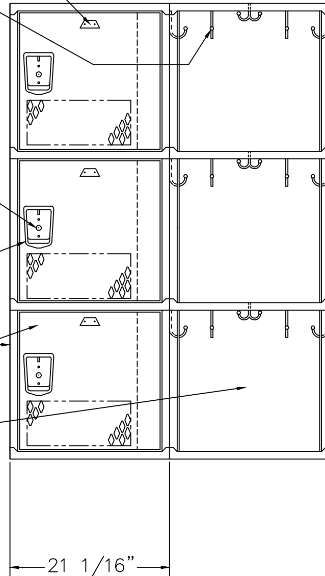
LOCKER ELEVATION
