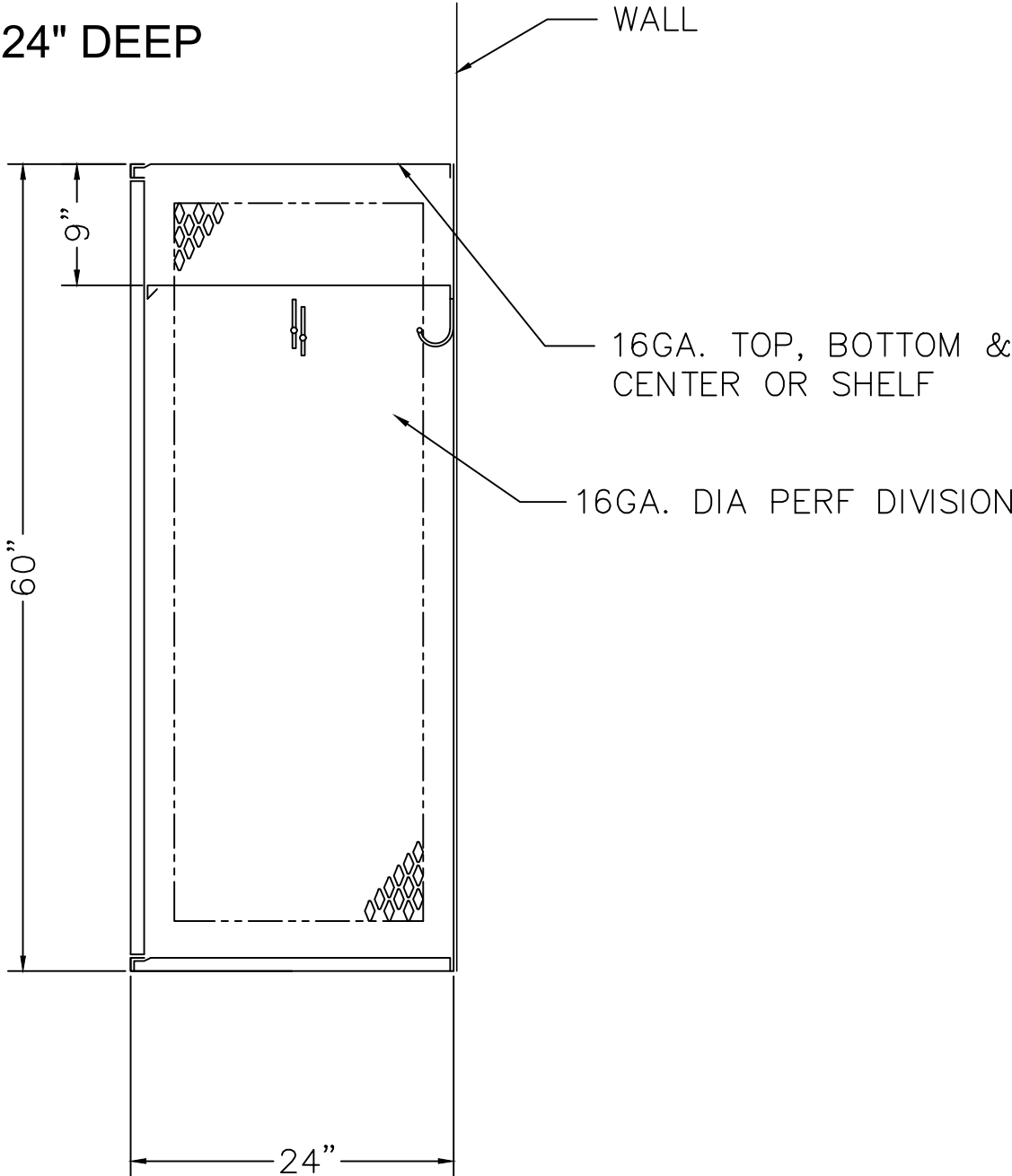
LOCKER SECTION
