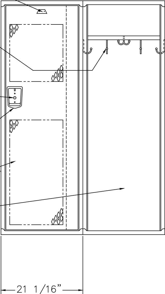
LOCKER ELEVATION
