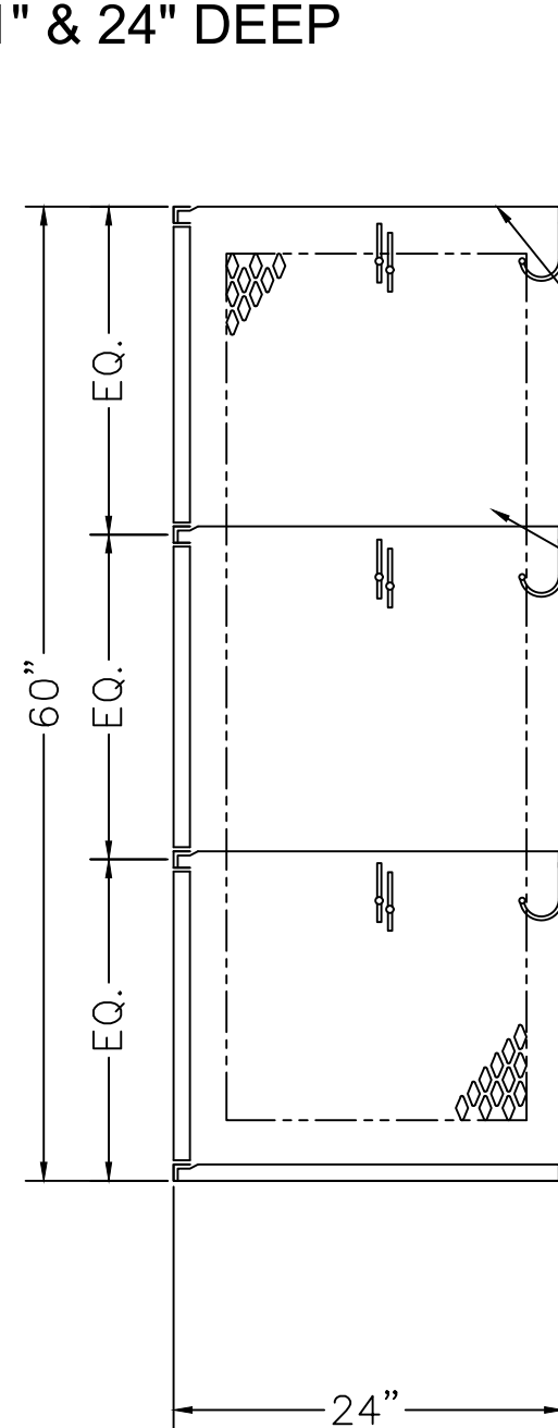
LOCKER SECTION
