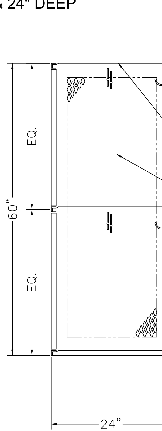
LOCKER SECTION
