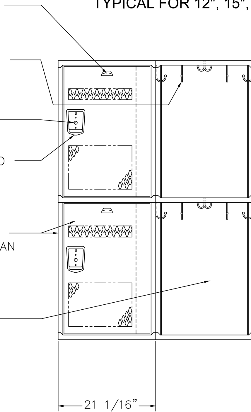
LOCKER ELEVATION
