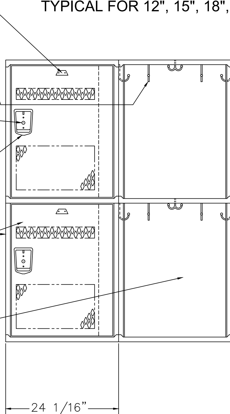
LOCKER ELEVATION
