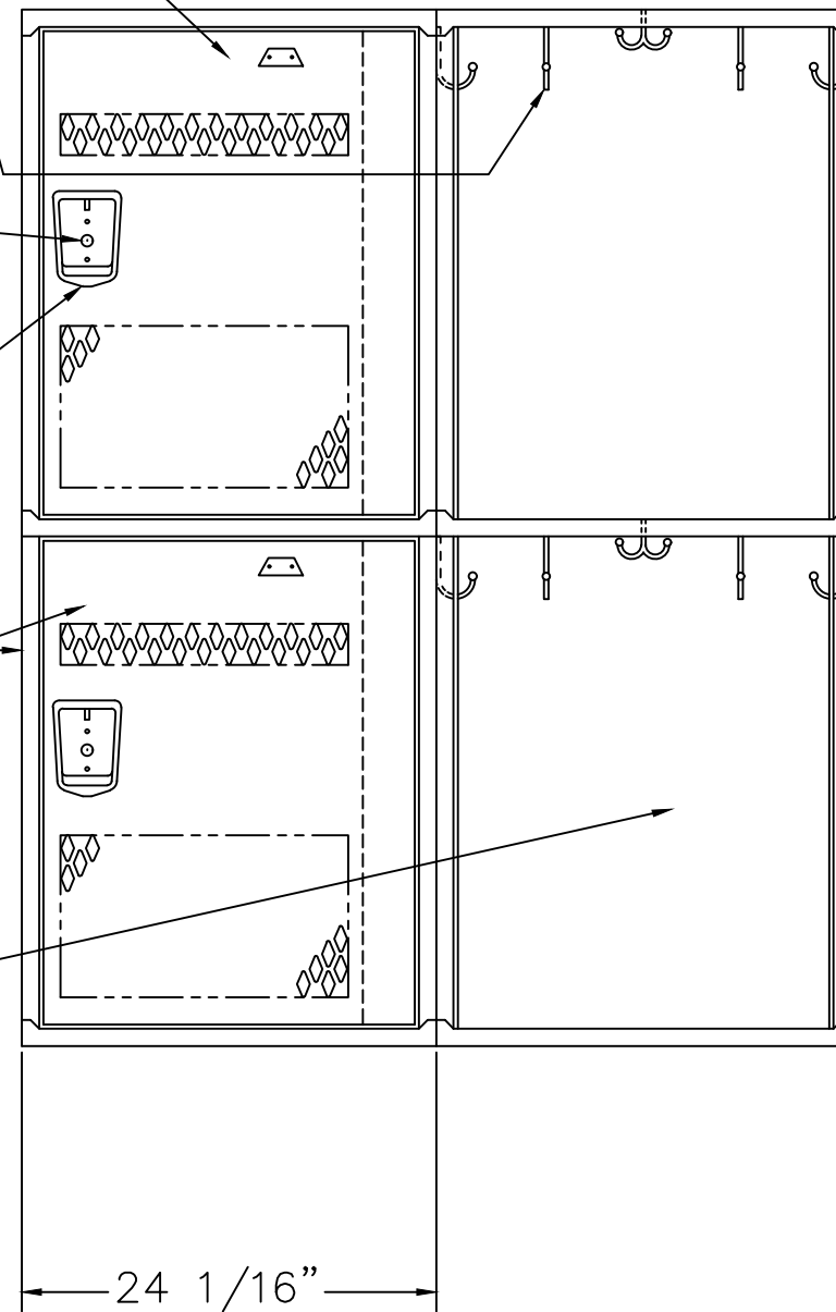
LOCKER ELEVATION
