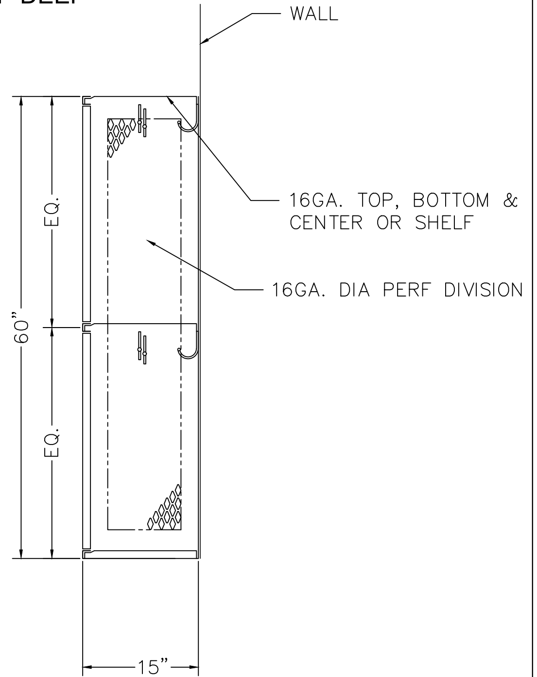
LOCKER SECTION
