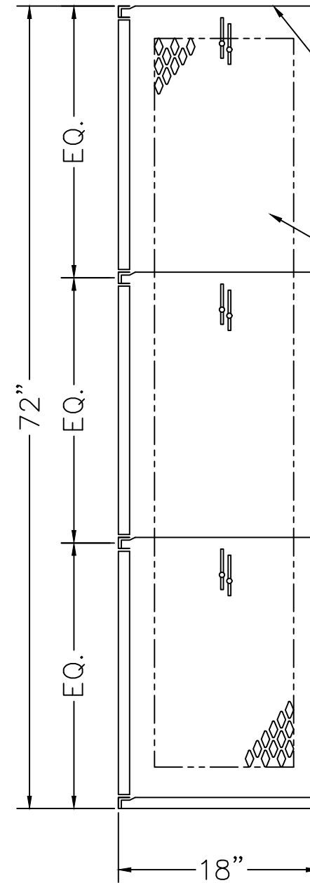
LOCKER SECTION
