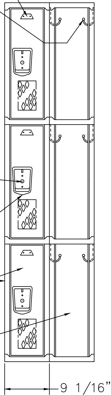
LOCKER ELEVATION
