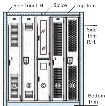
Front View of Locker with Recessed Trim
