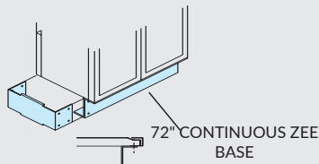
Zee Base (O) - Must use added support in rear of locker and in between groupings
