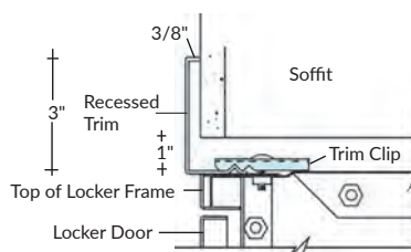
Side View of Top Recessed Trim
